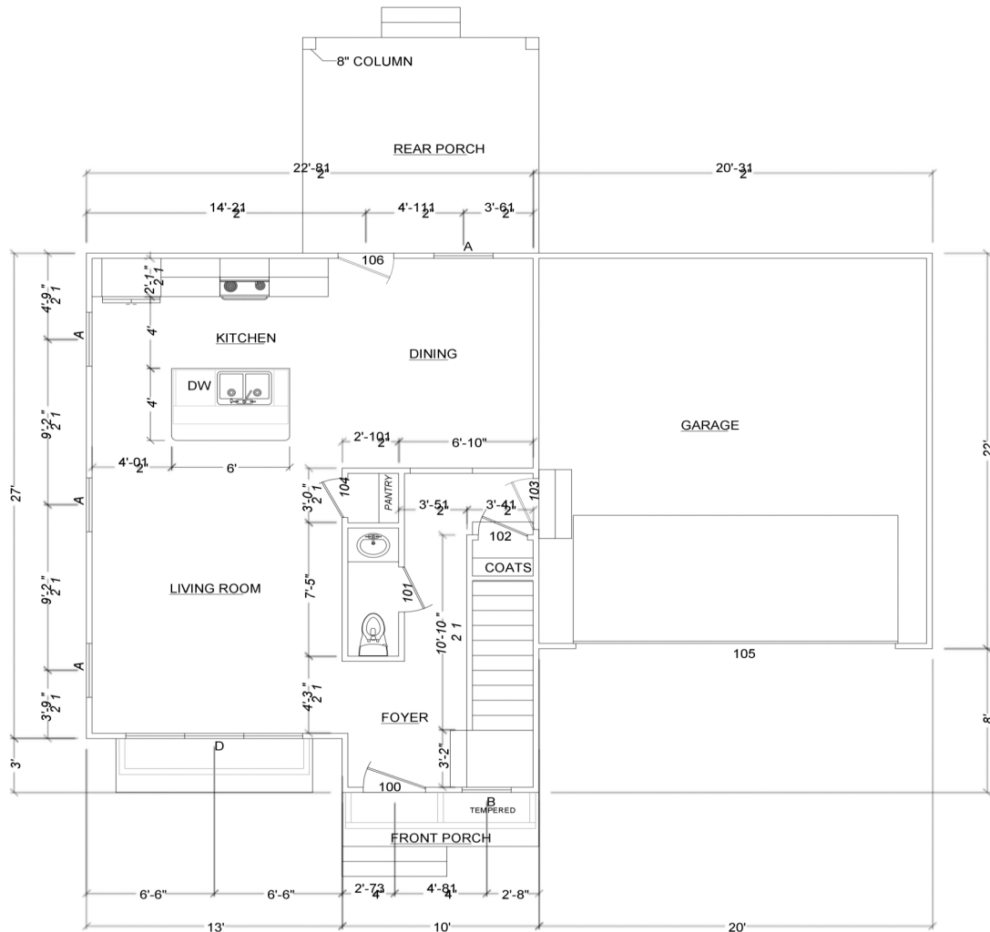
FLOOR PLAN - LEVEL 1
