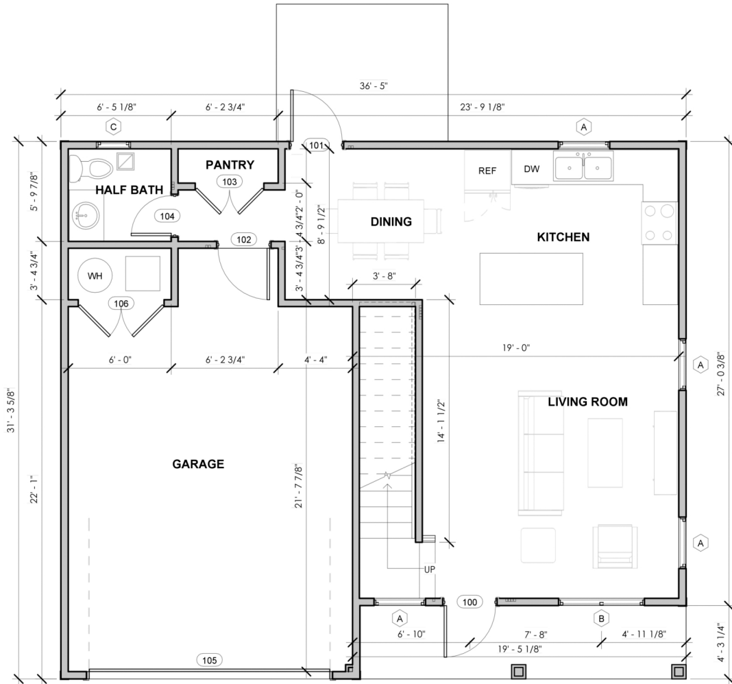
FLOOR PLAN - LEVEL 1
