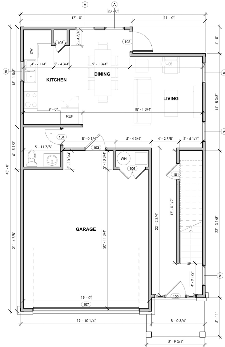
FLOOR PLAN - LEVEL 1
