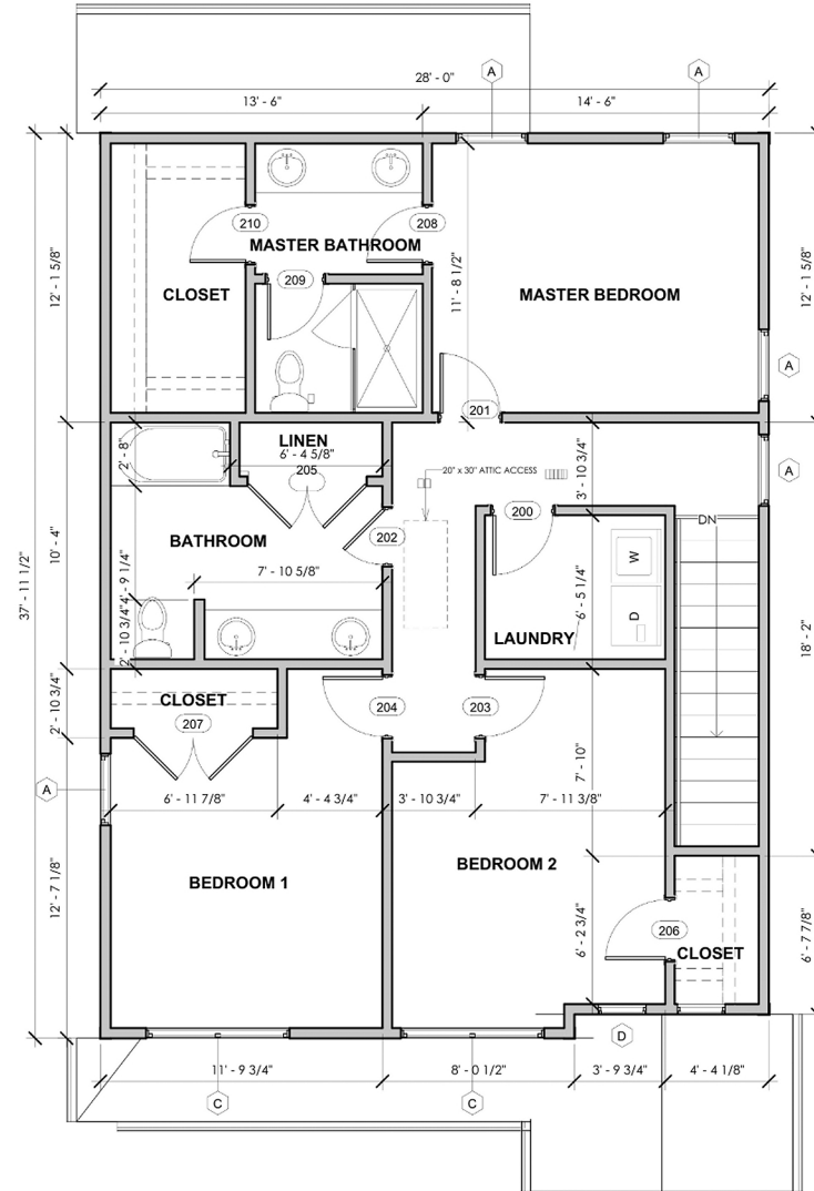
FLOOR PLAN - LEVEL 2
